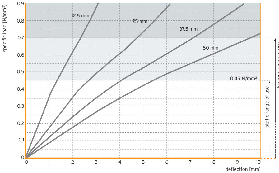
Figure 1: Quasistatic load deflection curve measured with a loading rate of 0.045 N/mm²/s
